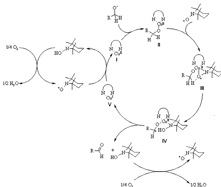
Figure 2. Proposed mechanism of (Cu-N-ligand-TEMPO)-catalysed oxidation of primary alcohols.
