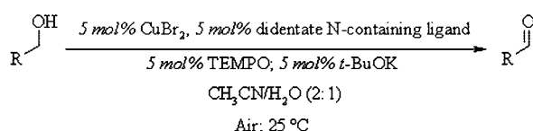
Figure 1. \text{CuBr}_2 -catalysed oxidation of primary alcohols.
