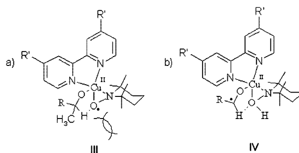
Figure 3. Possible explanations for the lack of reactivity of secondary alcohols: a) Steric hindrance due to the methyl group of the secondary alcohol preventing the formation of species III in the catalytic cycle; b) Stabilisation of the radical species IV by the second \beta -hydrogen of the primary alcohol.
